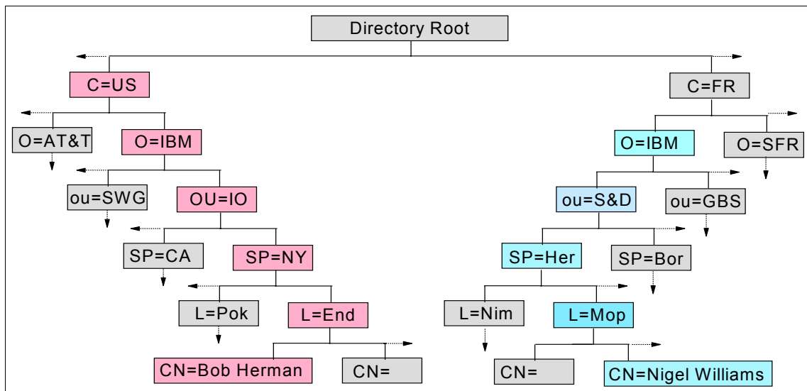
Figure 6-12 Distinguished names
