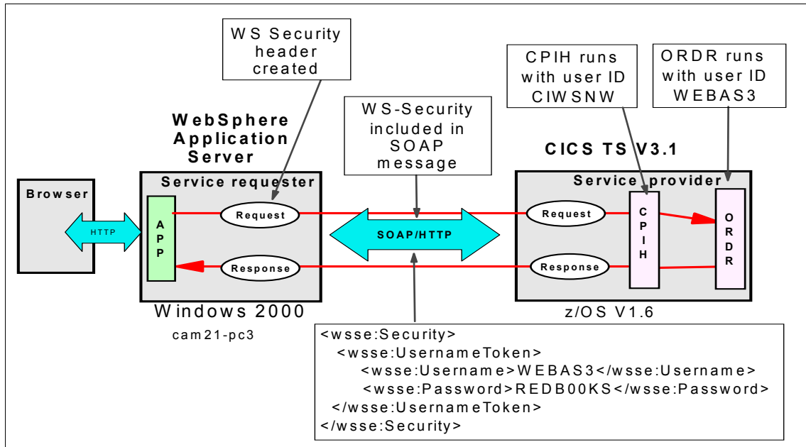
Figure 8-6 Enabling SOAP message security scenario
