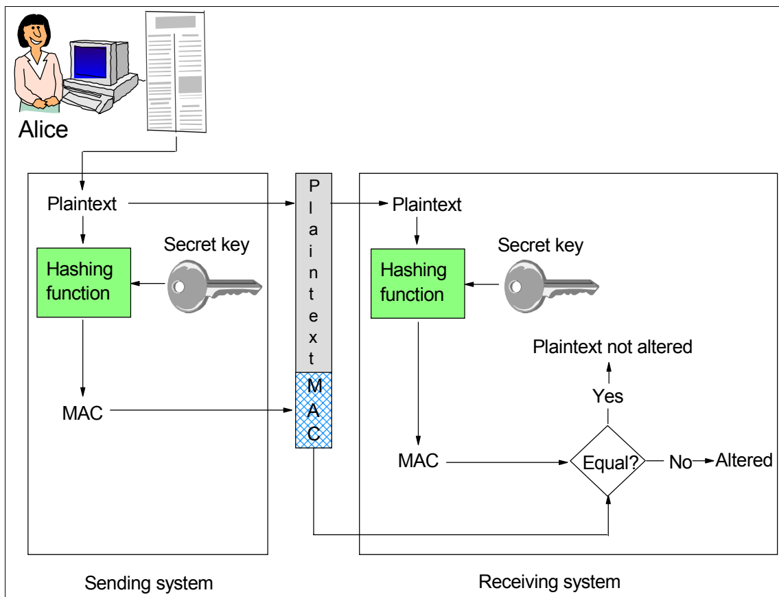
Figure 6-8 Keyed-hash message authentication code (HMAC)
