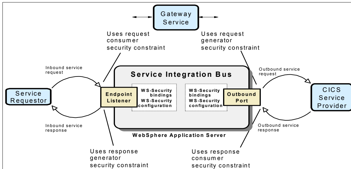
Figure 7-7 Securing a CICS Web service using the service integration bus
