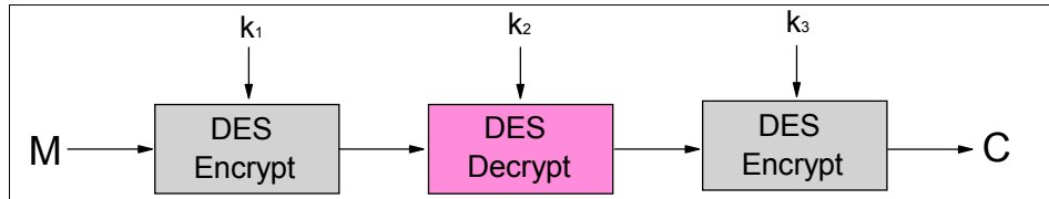
Figure 6-4 Triple DES - EDE
