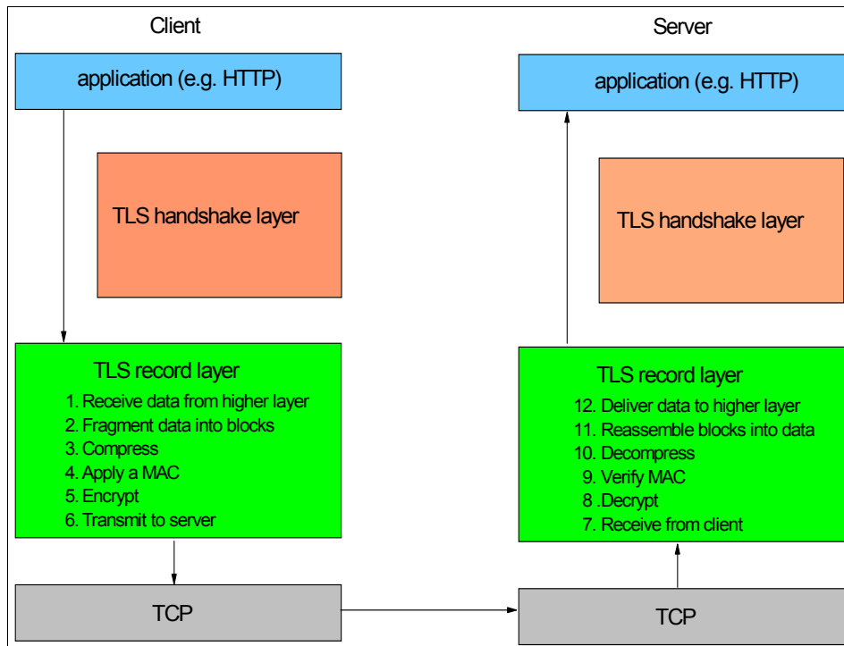
Figure 6-15 Overview of TLS
