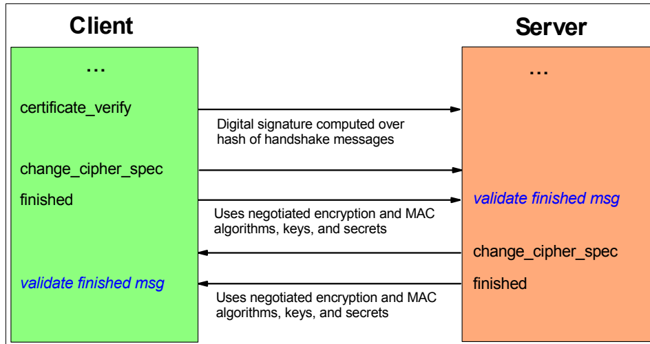
Figure 6-19 Starting a new TLS session (3): Verification
