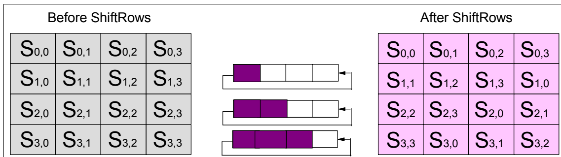
Figure B-4 ShiftRows() cyclically shifts the last three rows in the state array
