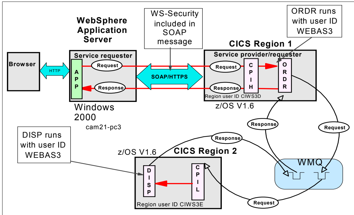
Figure 8-22 SOAP message security with WebSphere MQ scenario
