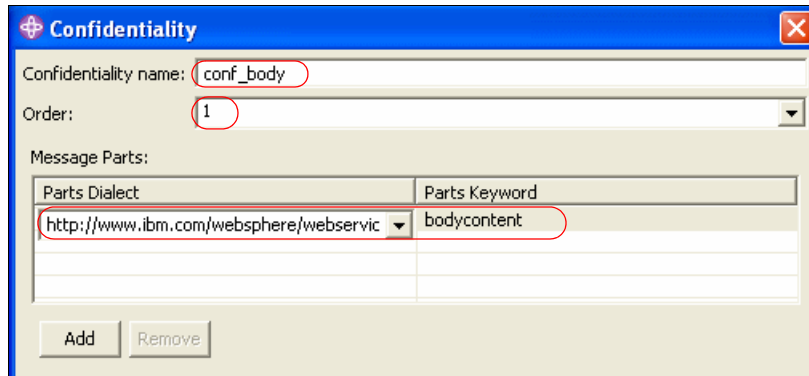
Figure 9-39 Confidentiality dialog in the WS Extensions page
