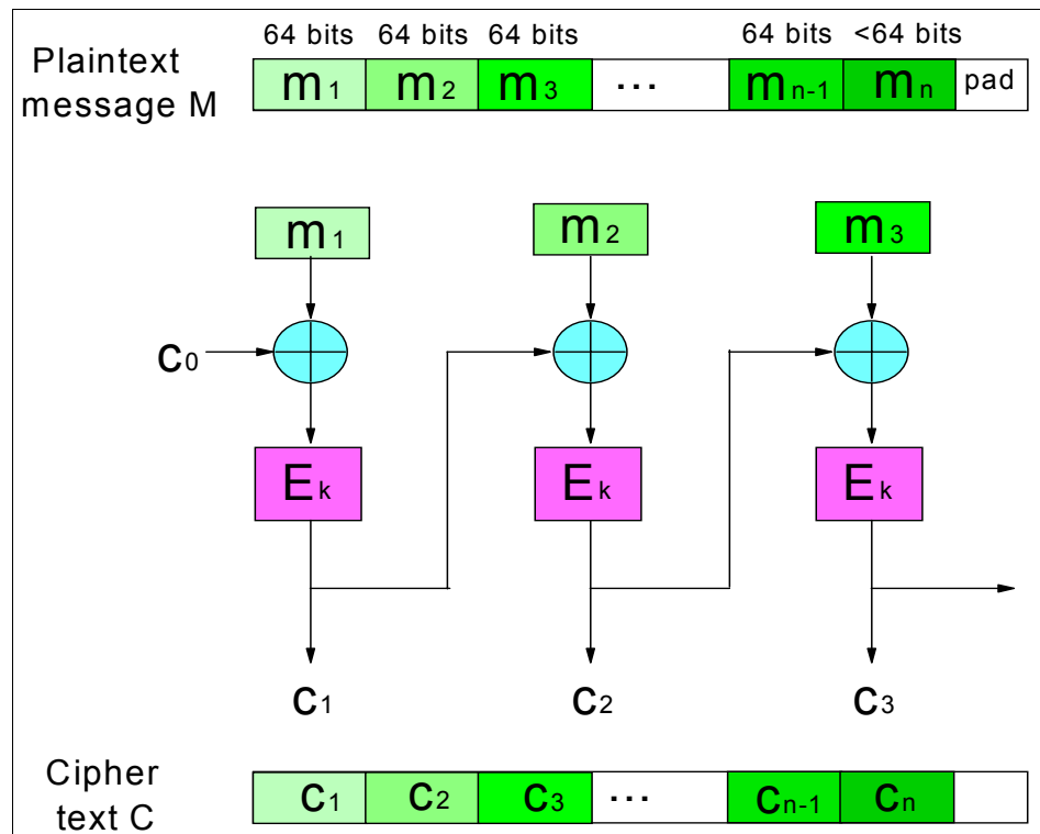
Figure 6-3 Cipher block chaining (CBC) mode of operation
