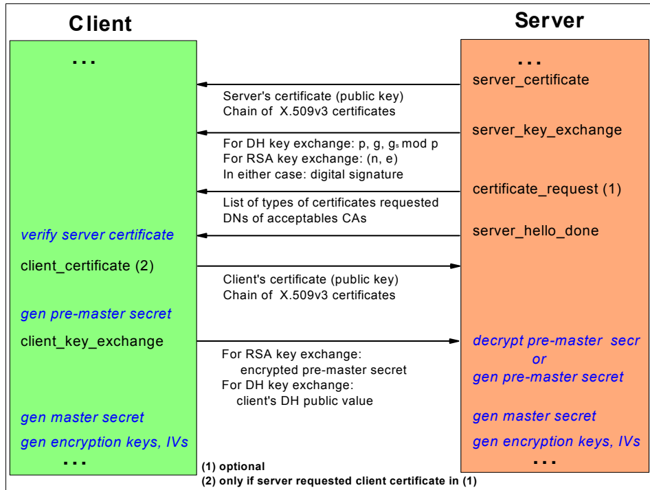
Figure 6-18 Starting a new TLS session(2): Establishing the pre-master secret
