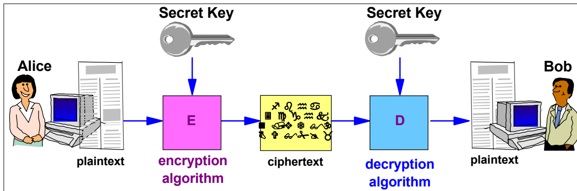
Figure 6-1 Secret key (or symmetric) cryptography
