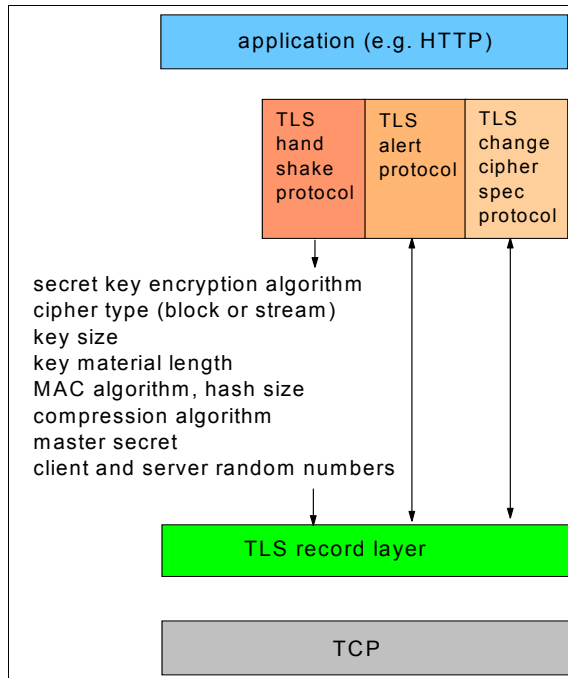
Figure 6-16 Handshake protocol passes security parameters to the record layer
