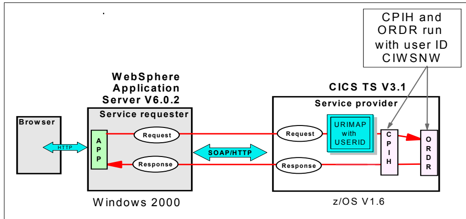
Figure 8-2 Setting user ID on a URIMAP scenario
