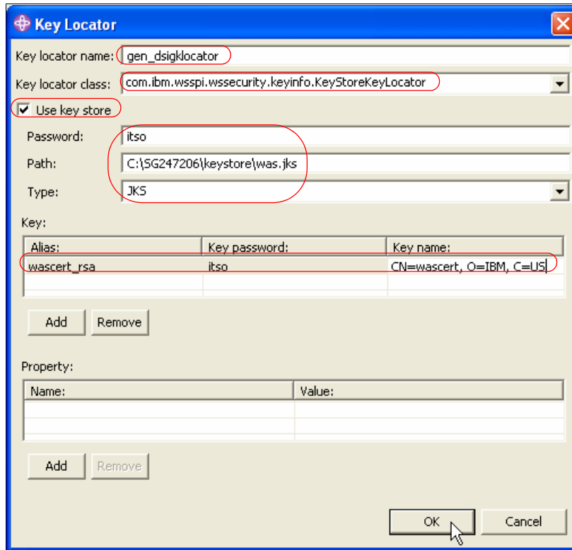
Figure 9-22 The Key Locator dialog in the WS Binding page
