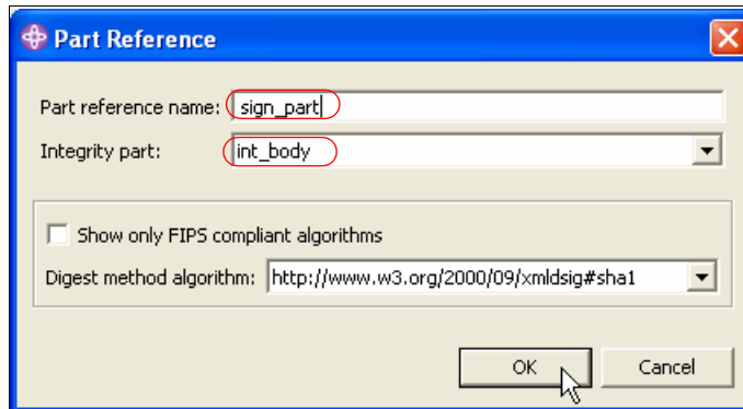
Figure 9-25 The Part Reference dialog in the WS Binding page
