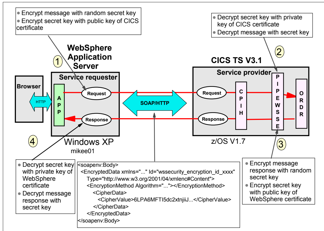
Figure 9-37 Enabling CICS WS-Security support for encryption
