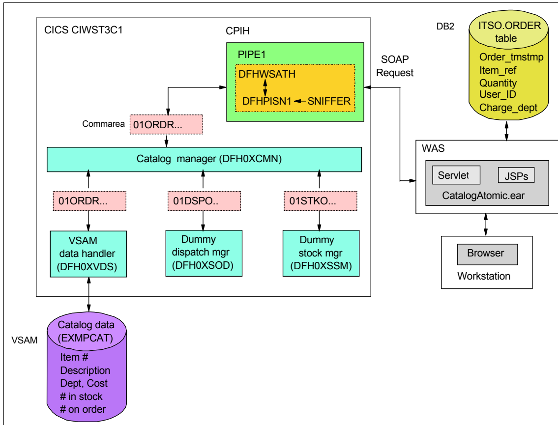
Figure 12-3 WebSphere as service requester and CICS as service provider
