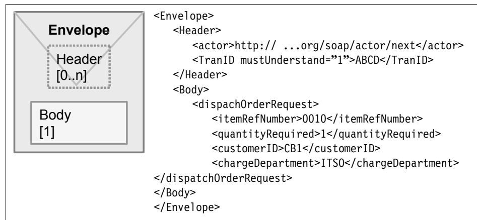
Figure 1-3 Example of a simple SOAP message
