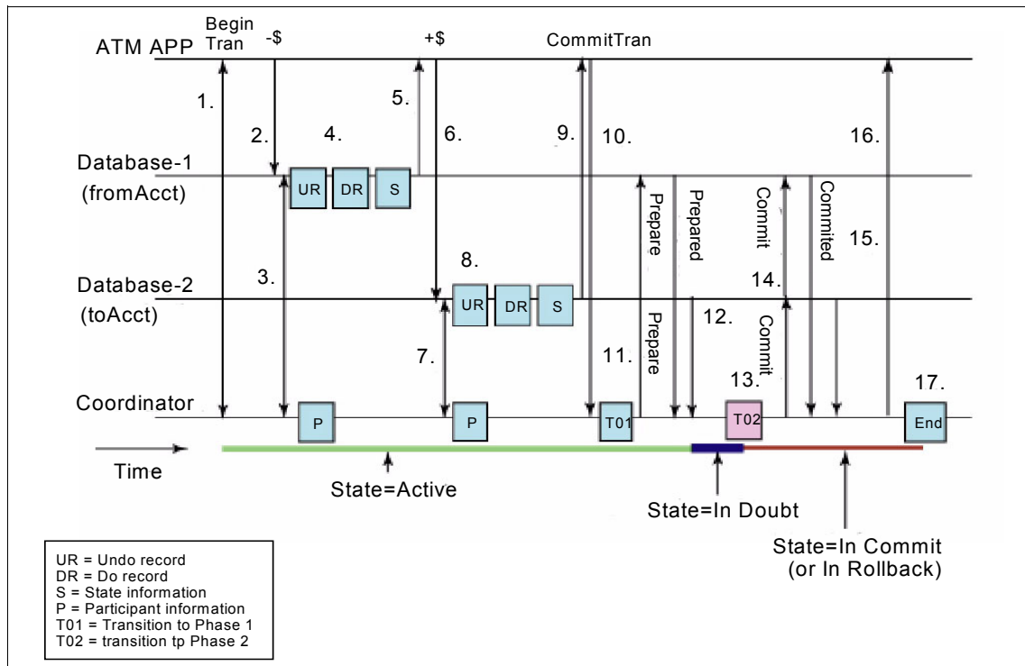
Figure 10-2 Behind the scenes of Waldo’s ATM transaction
