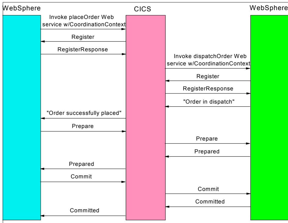
Figure 12-35 Successful daisy chain - Message flow
