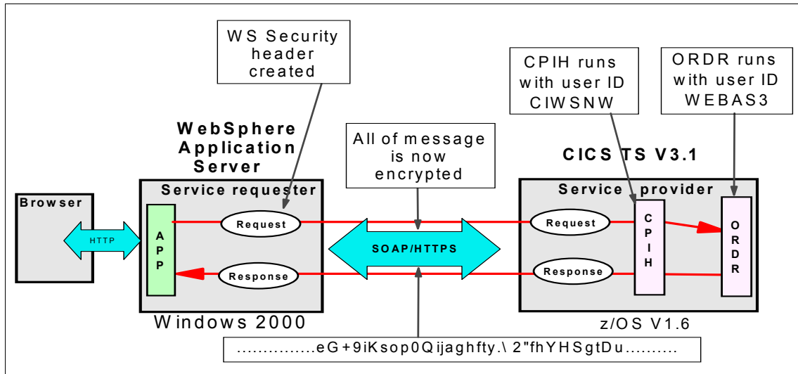
Figure 8-15 Enabling SSL/TLS scenario
