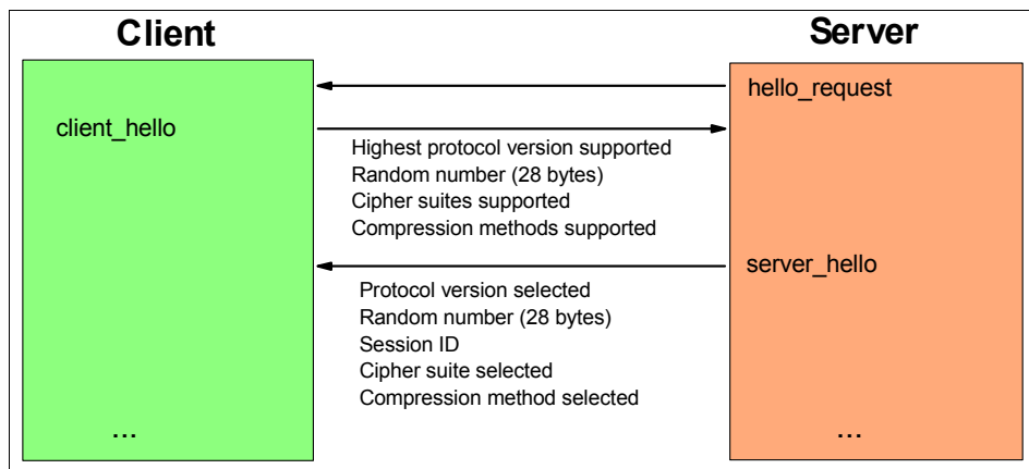
Figure 6-17 Starting a new TLS session(1): Establishing algorithms
