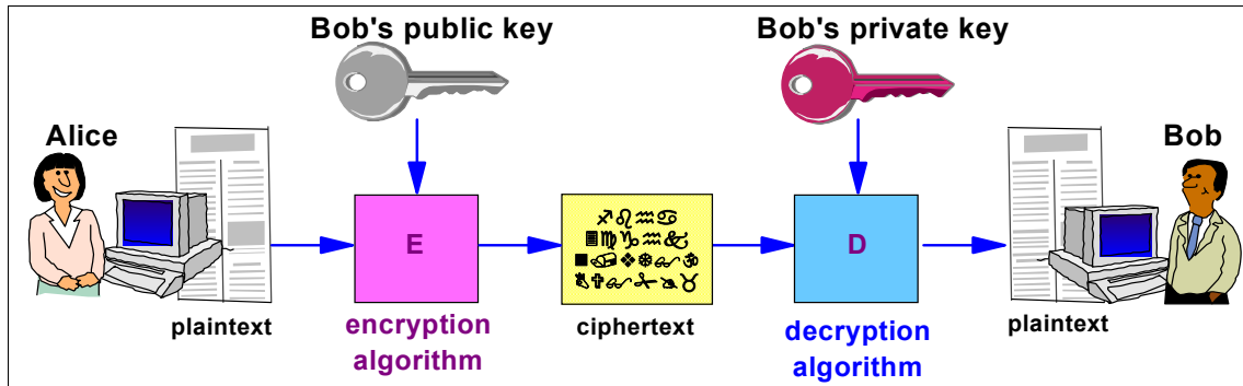
Figure 6-5 Public key (or asymmetric) cryptography
