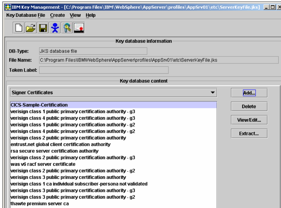
Figure 8-17 IKeyMan - After adding CICS CA certificate to keystore
