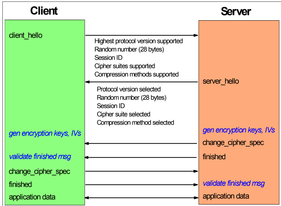
Figure 6-20 Resuming a session
