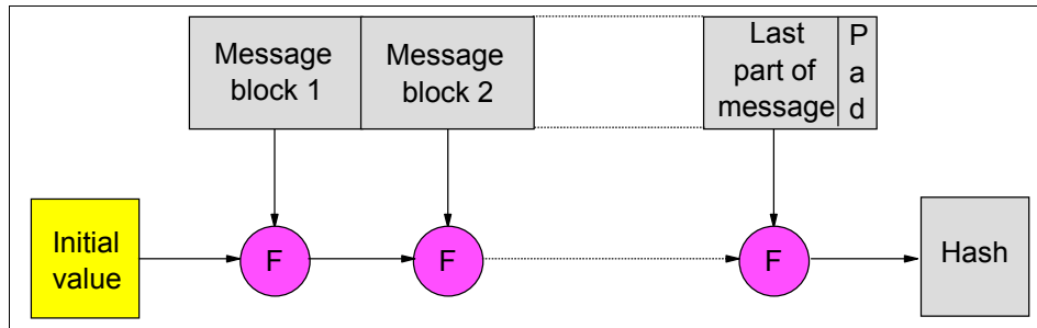
Figure 6-7 Iterative structure for hash functions
