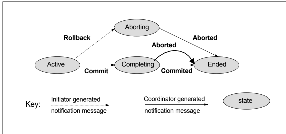
Figure 10-7 Completion protocol
