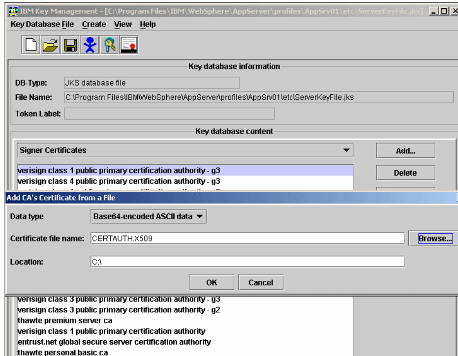
Figure 8-16 IKeyman - Add CICS CA certificate from an X509 file
