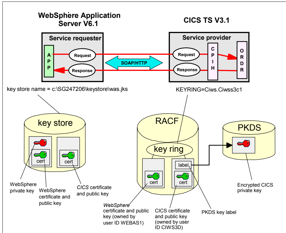
Figure 9-15 Certificates and key pairs used in signature and encryption scenarios
