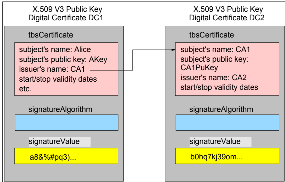
Figure 6-14 Certification path
