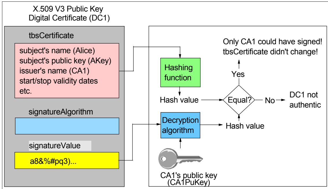
Figure 6-13 Verifying digital certificate
