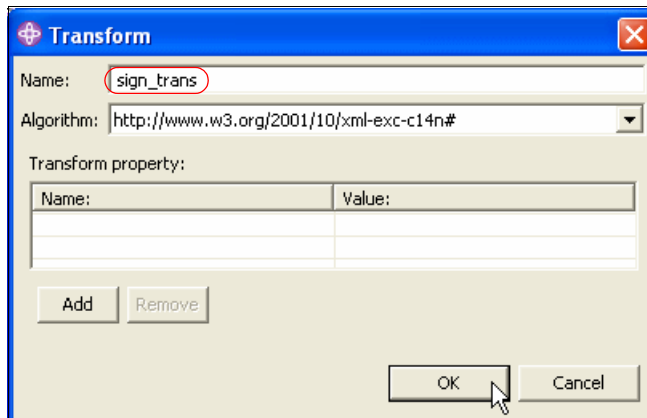
Figure 9-26 The Transform dialog in the WS Binding page
